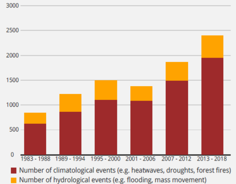
Figure 2 - Increase in number of extreme weather events 4
