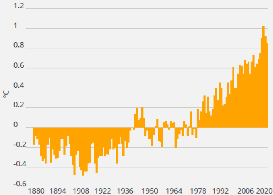
Figure 1 - Deviation in global temperature (°C) vs the 1951-1980 average
